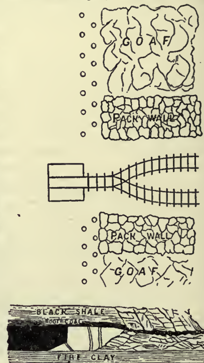
FIG. 10.—Long-wall working-face—Plan and Section.
